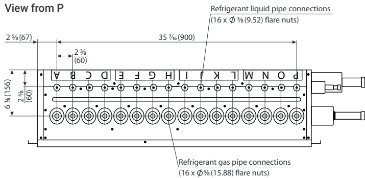
Indoor unit connecting side
