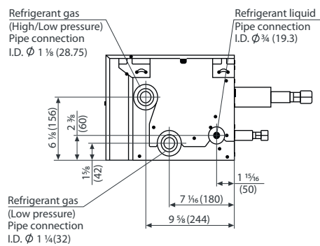
Outdoor unit connecting side
