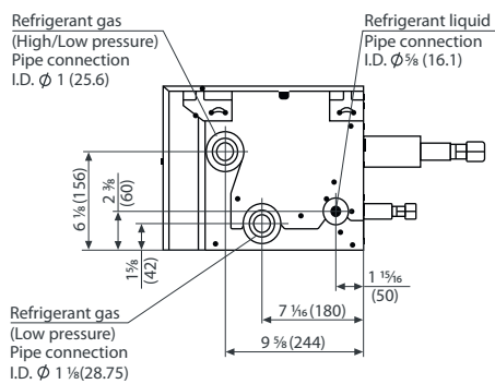
Outdoor unit connecting side
