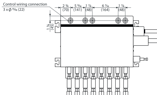
Outdoor unit connecting side
